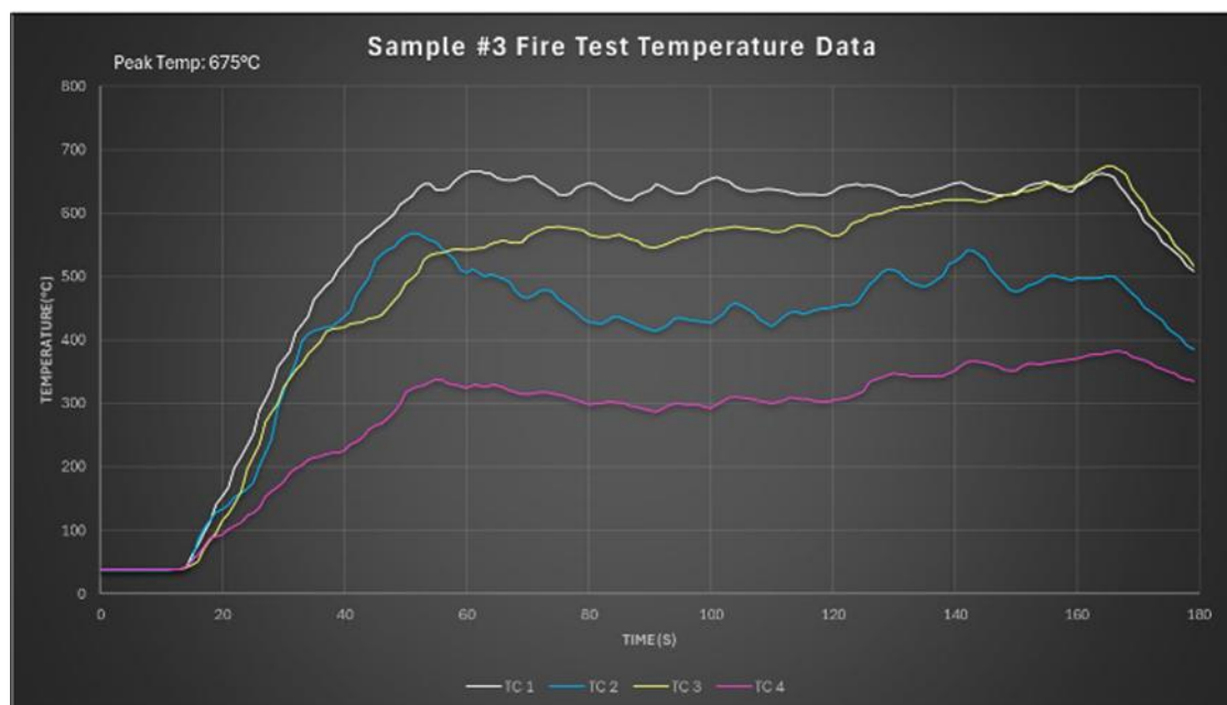
Sample #3 Fire Test Temperature Graph
